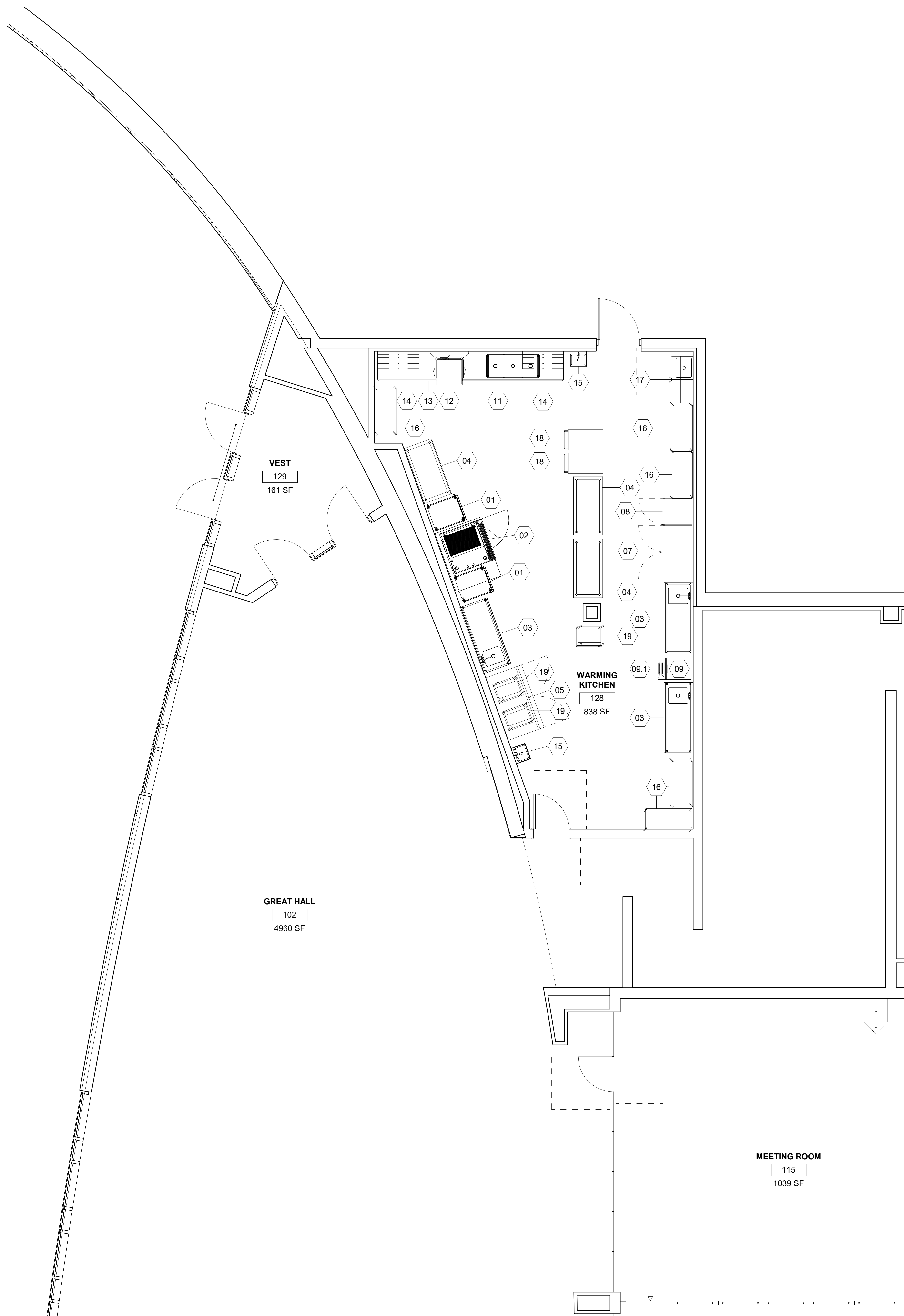
1 WARMING KITCHEN EQUIPMENT PLAN FS101 1/4" = 1'-0"
